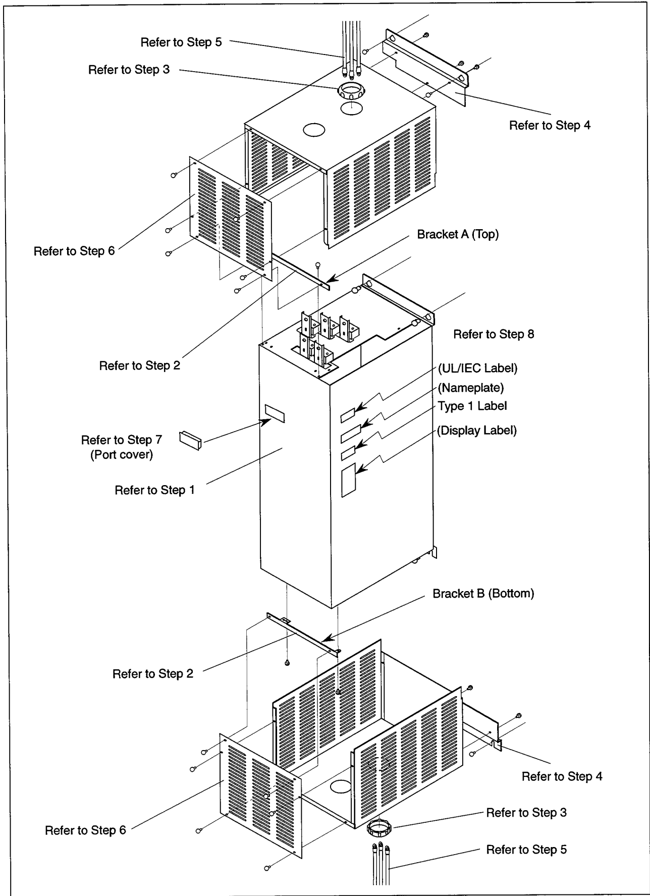
Figure 1 - Mounting NEMA Type 1 Kit to GV3000/SE Drive
