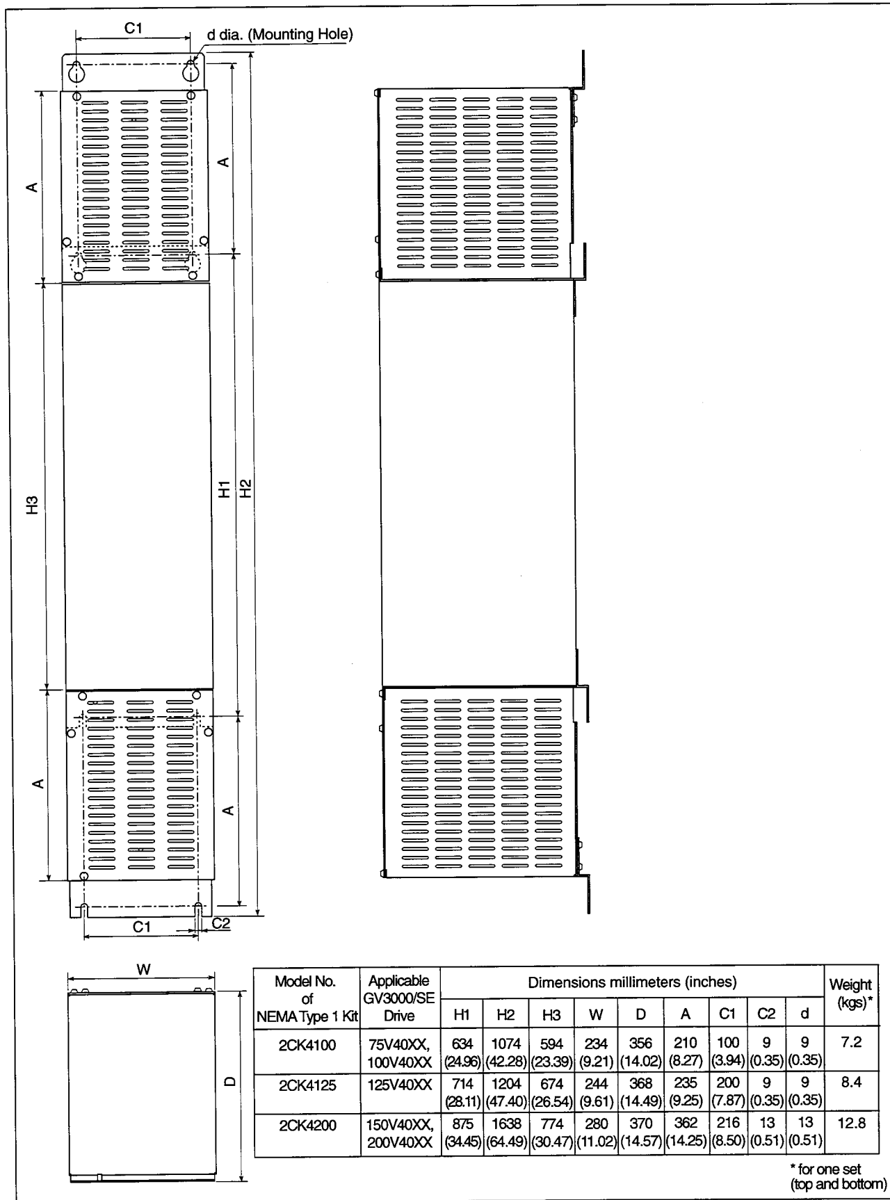
Figure 2 - Outline Dimensions of NEMA Type 1 Kit
